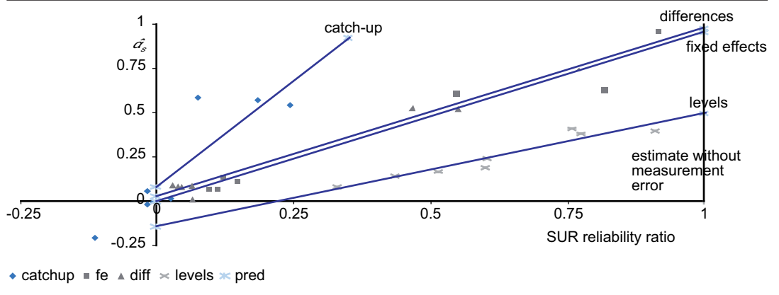
Figure 1 Estimated \alpha_s vs. SUR reliability ratio
