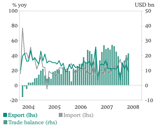
Chart 5: External trade
