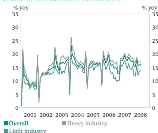
Chart 2: Industrial Production
