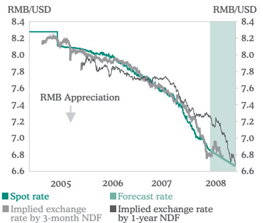
Chart 18: RMB appreciation
