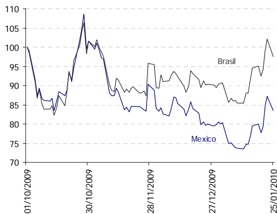
5-year CDS (01/10/2009=100)
